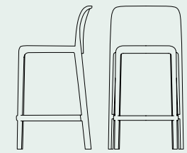
CB1984 | 47x46,5 H90 HS65 cm
